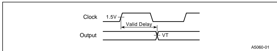
Figure 4. Setup and Hold Times
