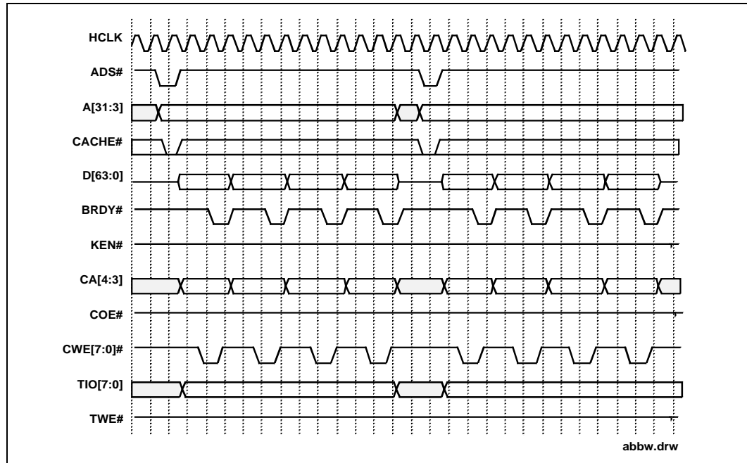
Figure 13. Read Miss, L2 Cache Write-Back, Line Fill, Standard SRAM
