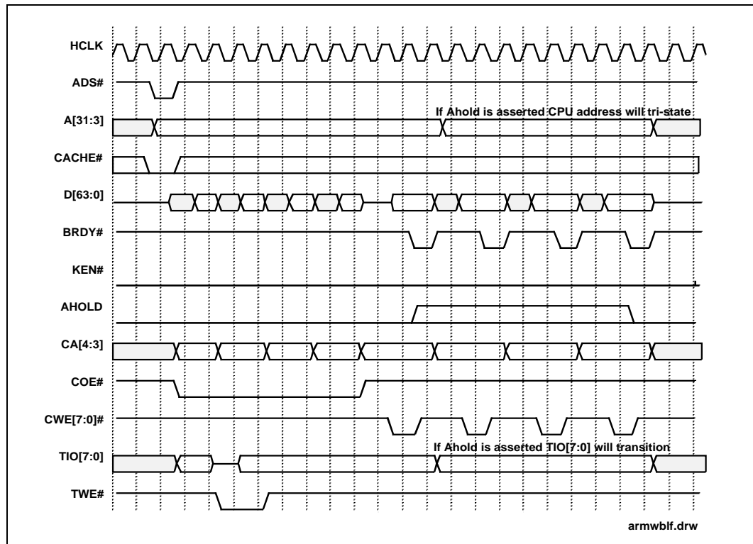
Figure 13. Read Miss, L2 Cache Write-Back, Line Fill, Standard SRAM
