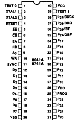
Figure 2. Pin Configuration
