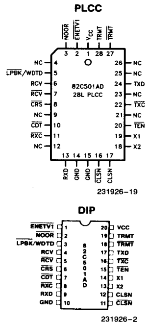
Figure 2. Pin Configurations (PLCC and DIP)
