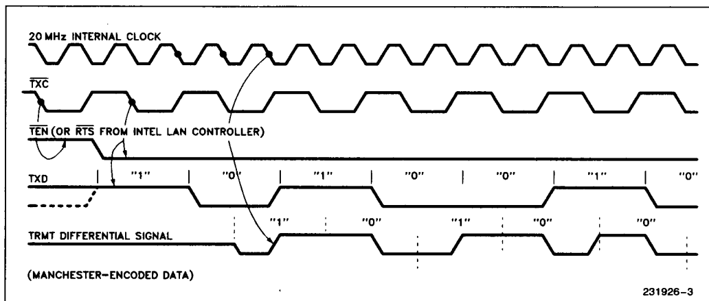
Figure 3. Start of Transmission and Manchester Encoding
